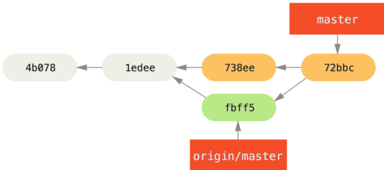
Figure 59. John's repository after merging origin/master .
