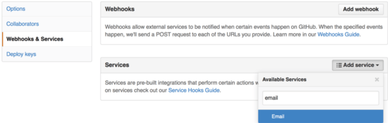
Figure 130. Sección Services and Hooks.
